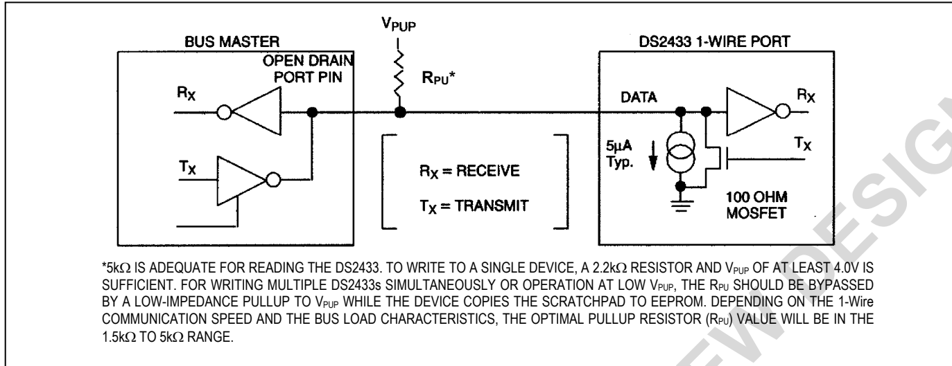
Figure 8. HARDWARE CONFIGURATION
